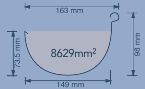
HALF ROUND UNSLOTTED
