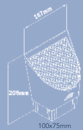
LEAF DIVERTER 100 X 75MM
